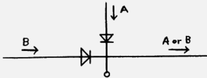
The OR Function
