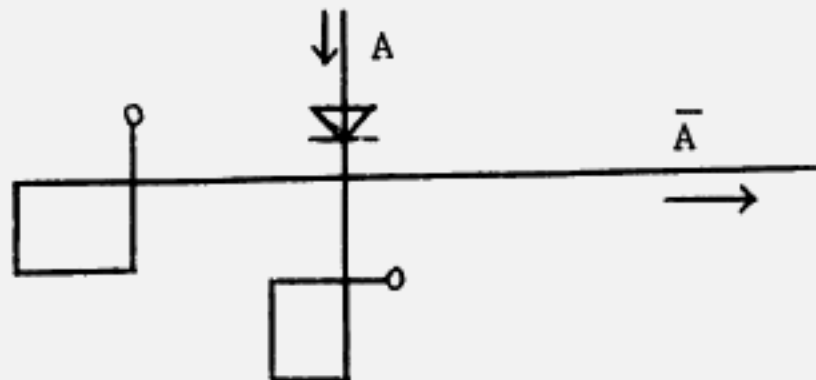
The NOT Function
