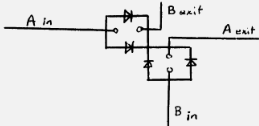
The Passive Crossover
